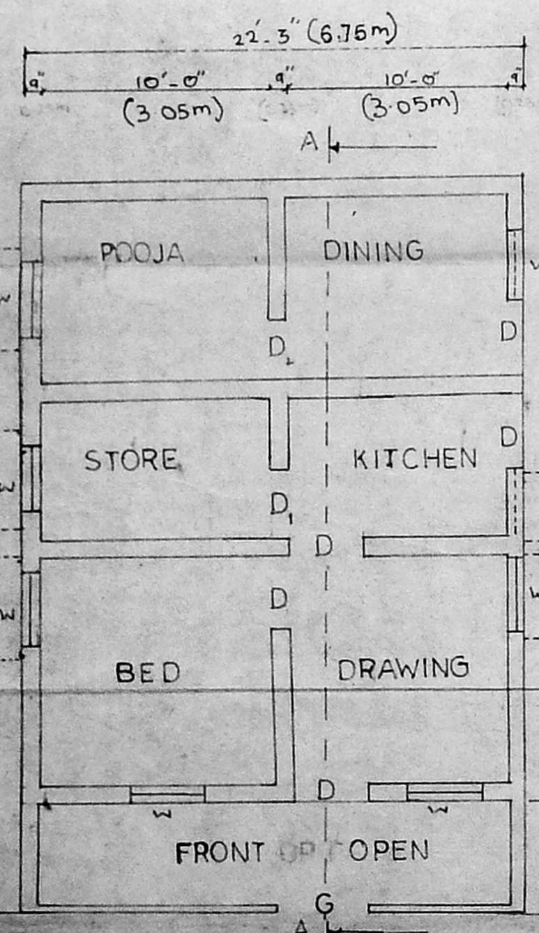
EXTG - GROUND FLOOR PLAN
