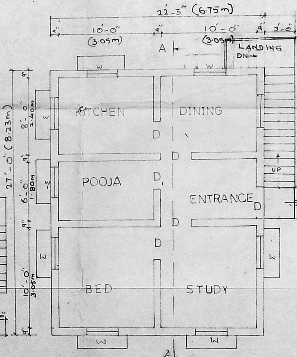
EXTG - FIRST FLOOR PLAN
