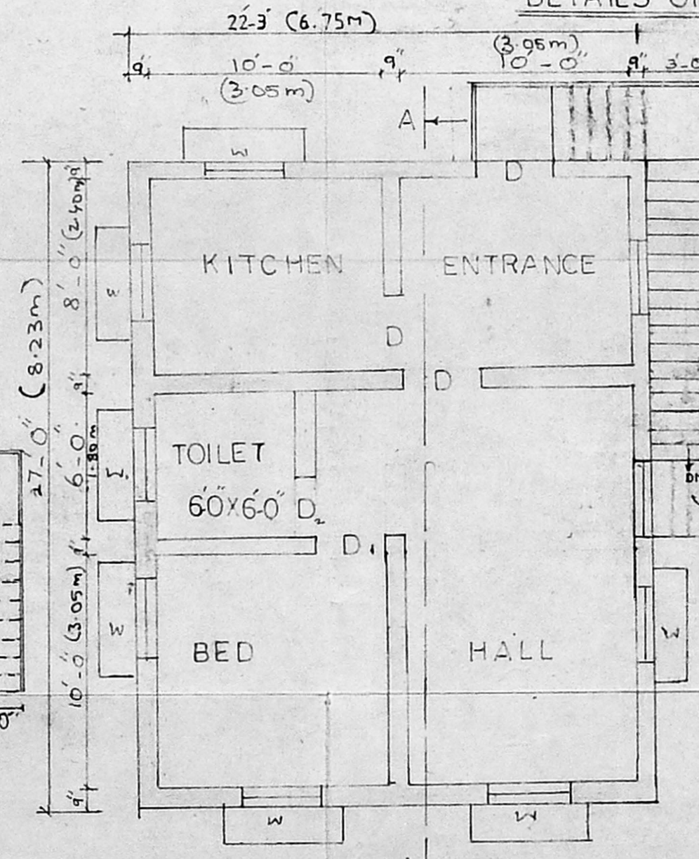
PRO - SECOND FLOOR PLAN
